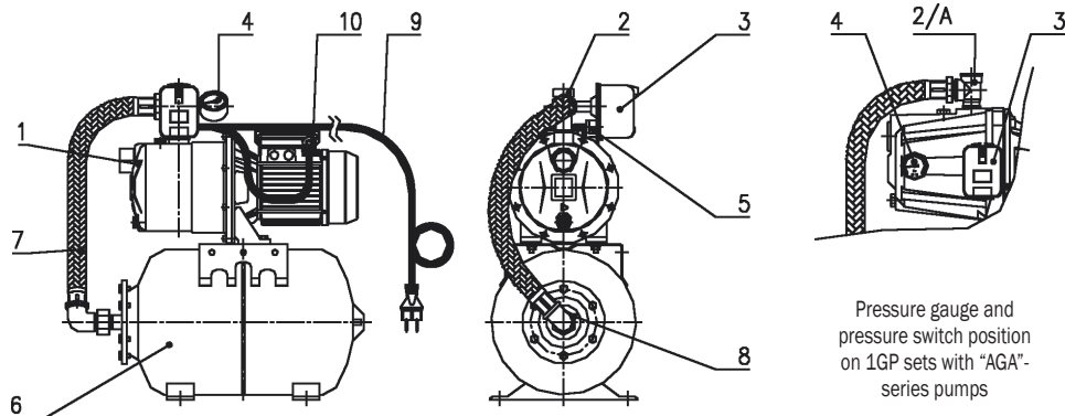
FIG. 6 Standard 1 GP set
